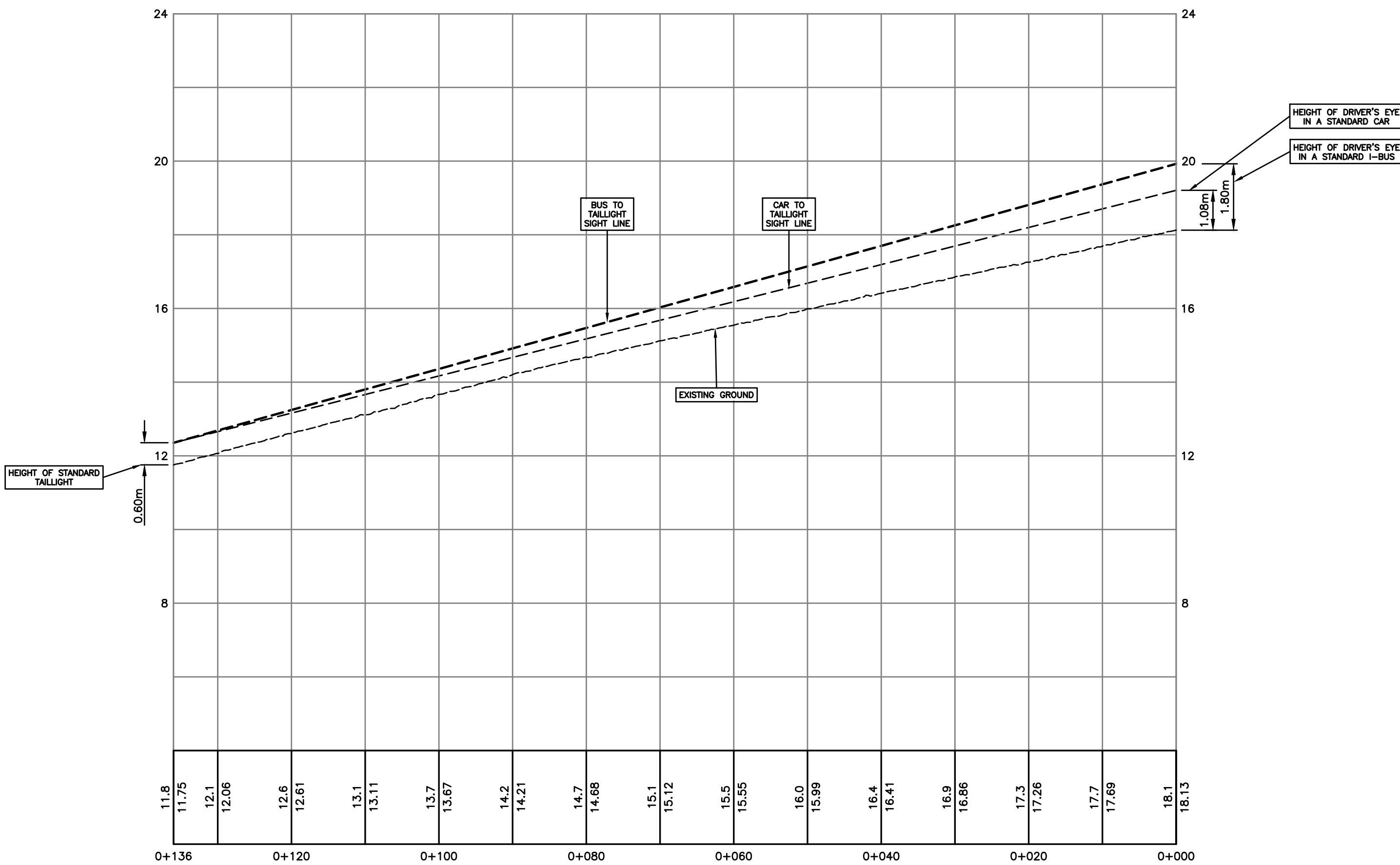
80KM/HR STOPPING SIGHT LINE
