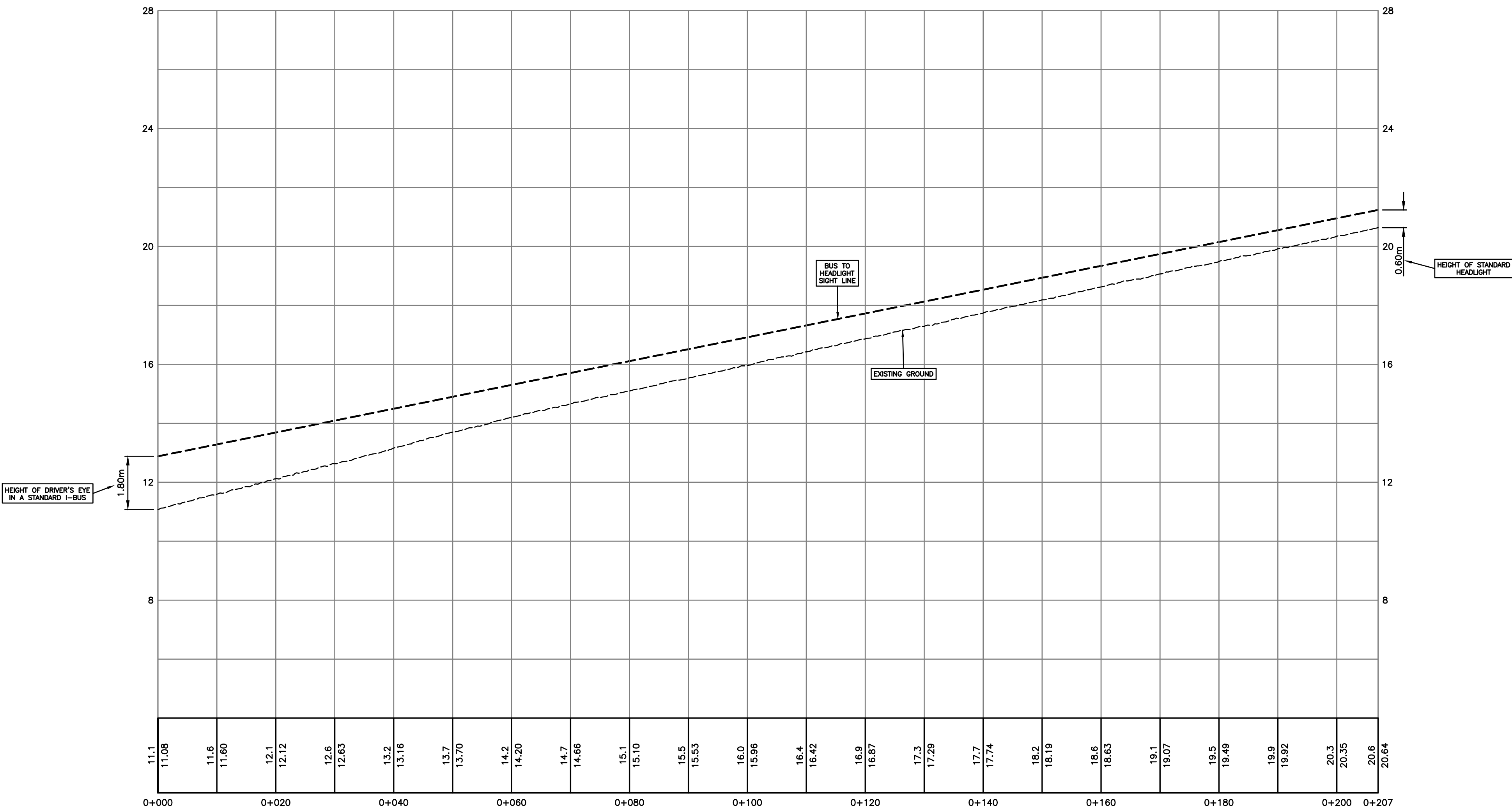
80KM/HR BUS MERGING SIGHT LINE
