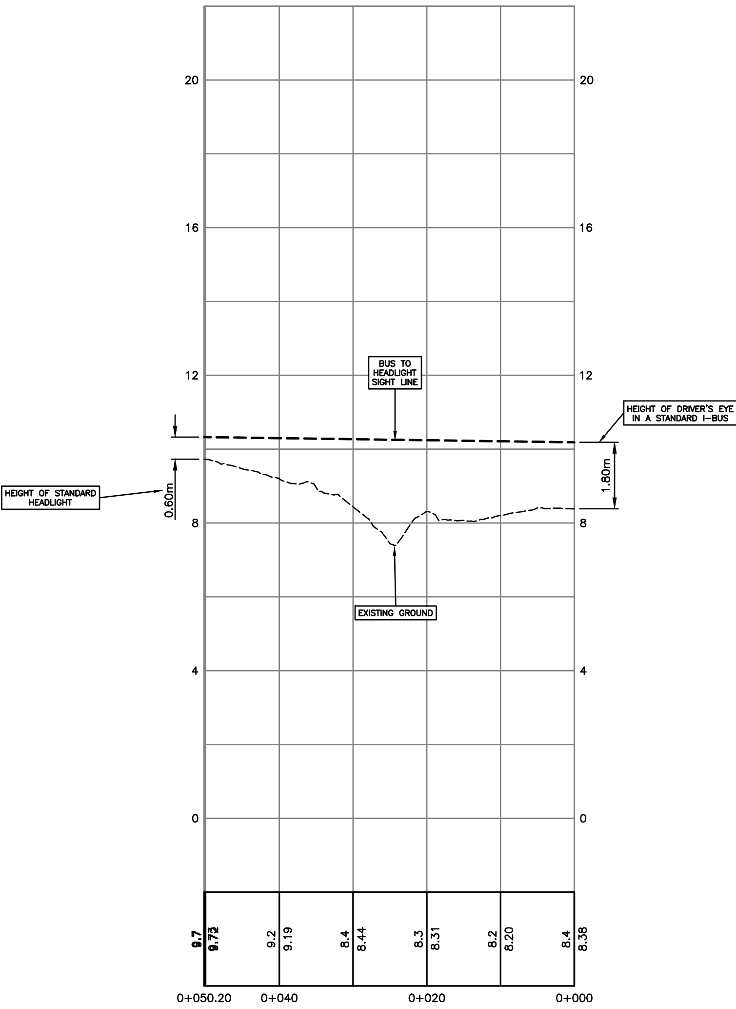
30KM/HR BUS MERGING SIGHT LINE
