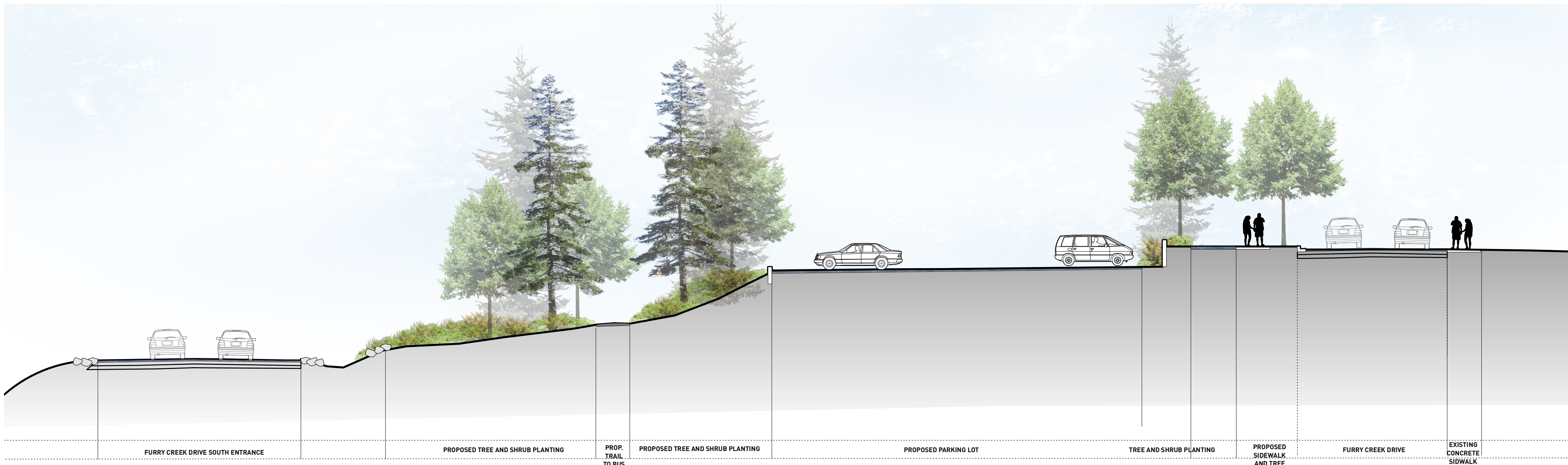
1 INTERCHANGE SOUTH Scale: 1:150
